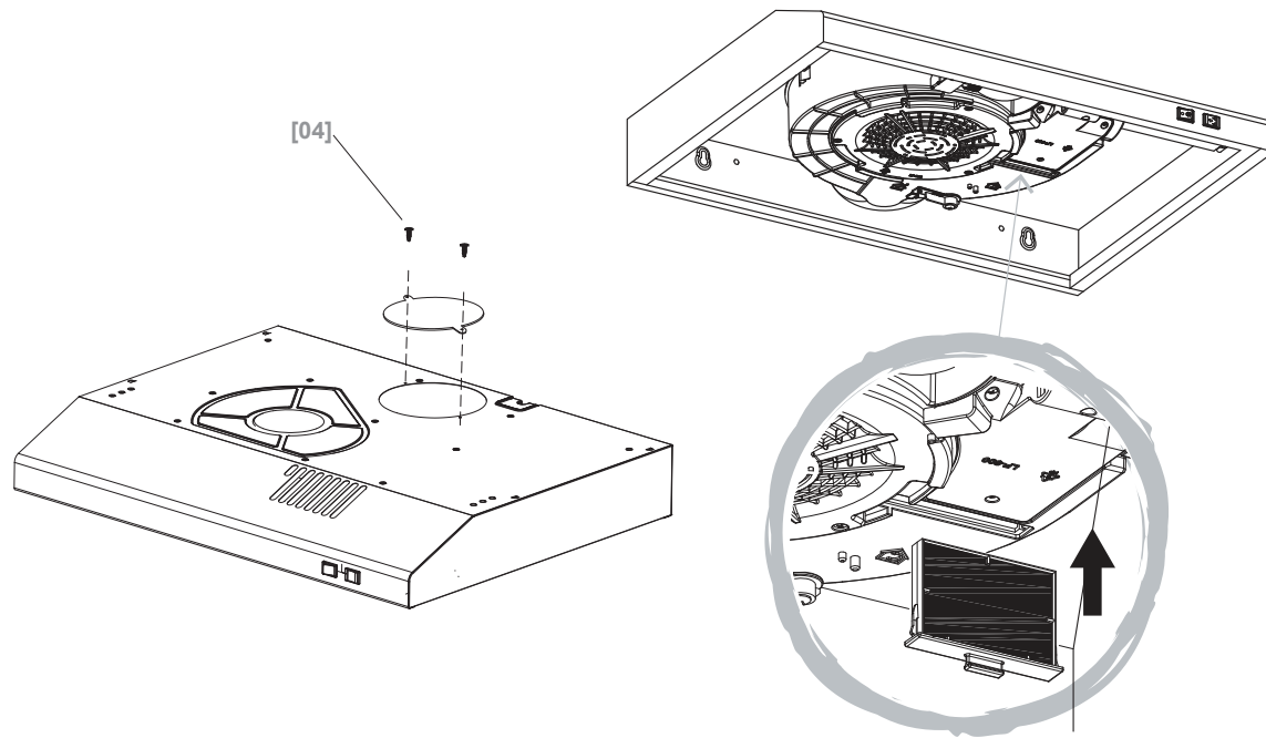
[04] x2 Ø3.5 x 10mm
